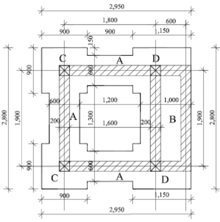
FOUNDATION PLAN
