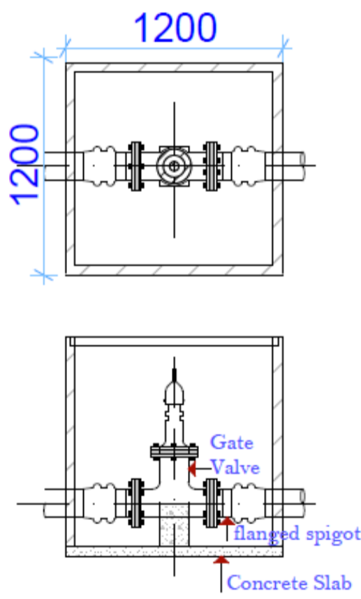
SLUICE VALVE Plan & Cross Section of Sluice Valve Chamber
