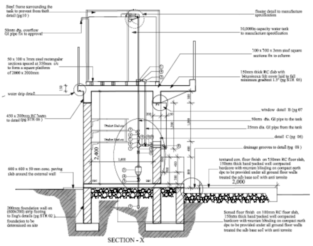
SECTION - X
