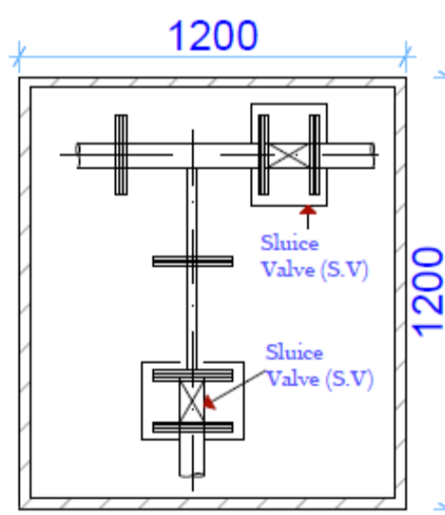
Plan of Junction Valve Chamber
